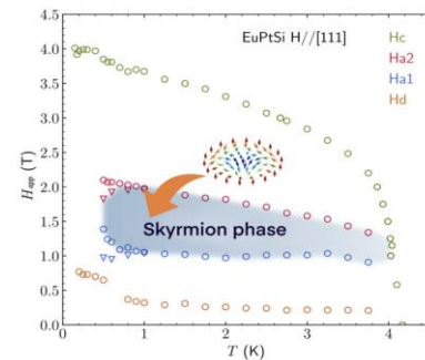
FIG. 1: Phase diagram of the chiral antiferromagnet EuPtSi exhibiting a skyrmion phase at low temperature, inside an antiferromagnetic phase.
