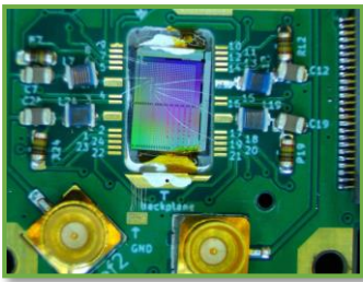
Si chip bonded for RF measurements
